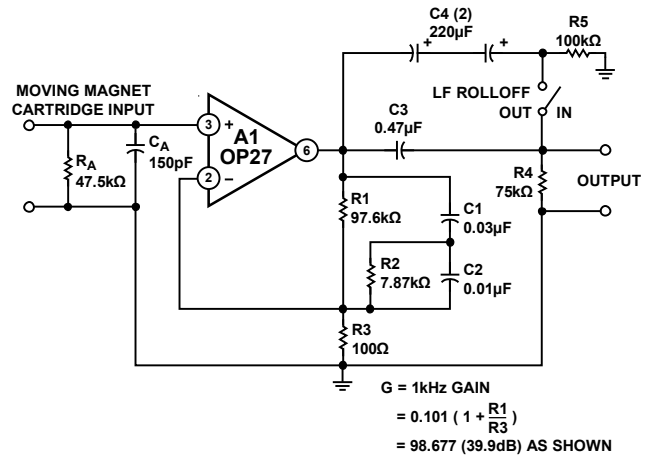
Figure 41. Phono Preamp Amplifier Circuit
